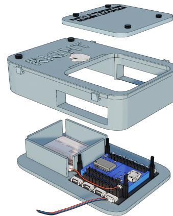
Figure 3: Exploded view of a sensory extension device control unit.
